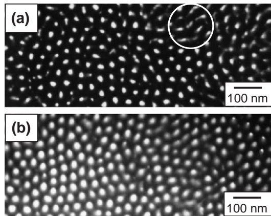
Fig. 2. Planar TEM images of the APA templates with 25 nm nanopores formed at different growth temperatures: (a) 27 and (b) 5 °C. The anodizing process of the Al/Si system was conducted under a constant voltage of 20 V, a sulfuric acid concentration of 15 wt.%, and an Al film thickness of 0.44 \mu\text{m} .
